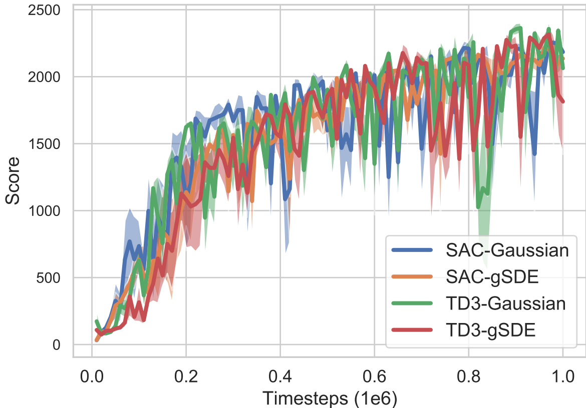
Walker2DBulletEnv-v0
