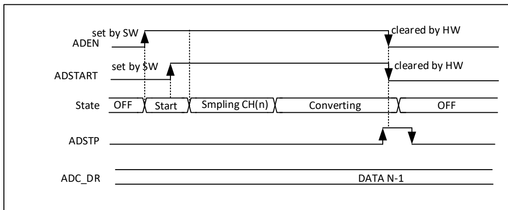
图 13-5 Stop timing
