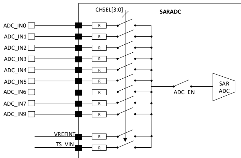
图 13-1 ADC channel with analog switch
