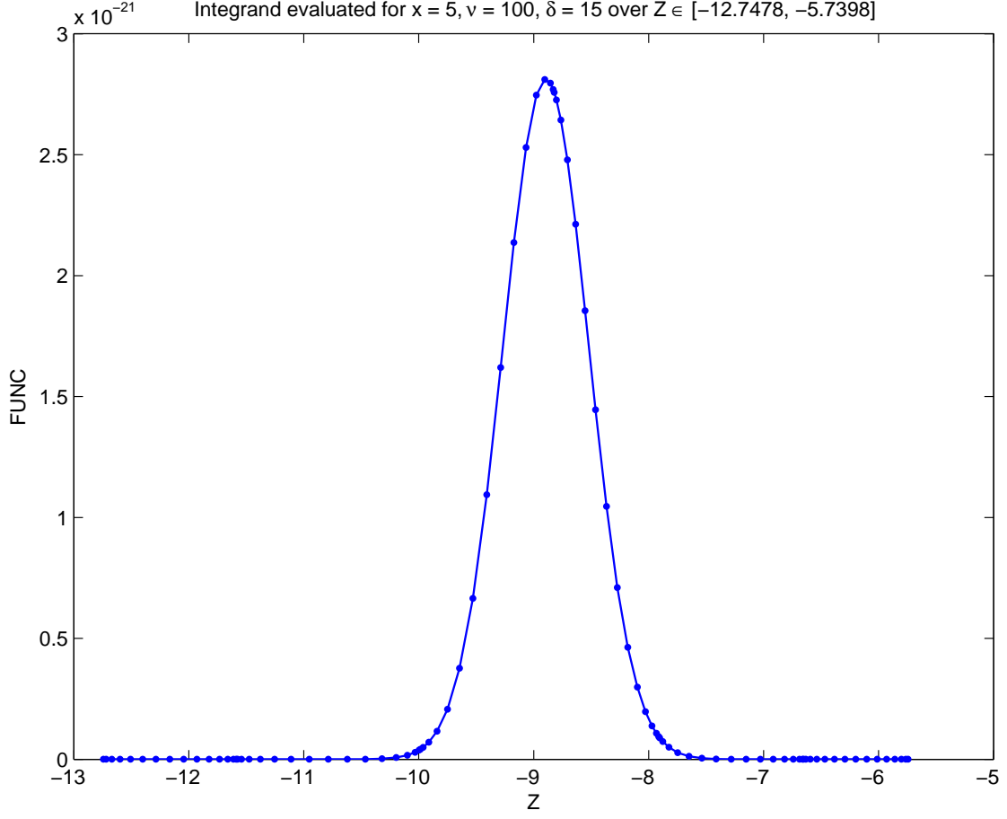
Figure 1: The integrand function g(z) evaluated at the Gauss-Kronrod nodes ( 90 = 6 subintervals \times 15 nodes) and the selected integration limits [A, B] used for computing the CDF of the noncentral t -distribution with the input parameters x = 5 , \nu = 100 and \delta = 15 . The value of CDF computed by the algorithm nctcdfvw is \text{CDF} = 2.640405806735035 \times 10^{-21} . For comparison, the standard MATLAB function nctcdf (Statistics Toolbox) returns \text{CDF} = 4.542511227039881 \times 10^{-43} , the R function pt returns \text{CDF} = 2.35515251660662 \times 10^{-21} , the SAS function probt returns \text{CDF} = 2.6404058074408 \times 10^{-21} , and the BOOST function non_central_t returns \text{CDF} = 2.64040580673507 \times 10^{-21} .
