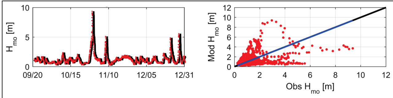
Figure 3. Example of scattered data (phase lag of 24 hr) that yield a bias and symmetric regression of approximately 0.0 and 1.0, respectively.
