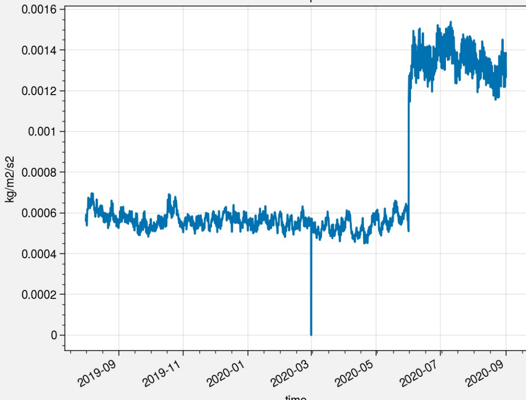
Upward moist convective mass flux: Global full atmosphere mean
