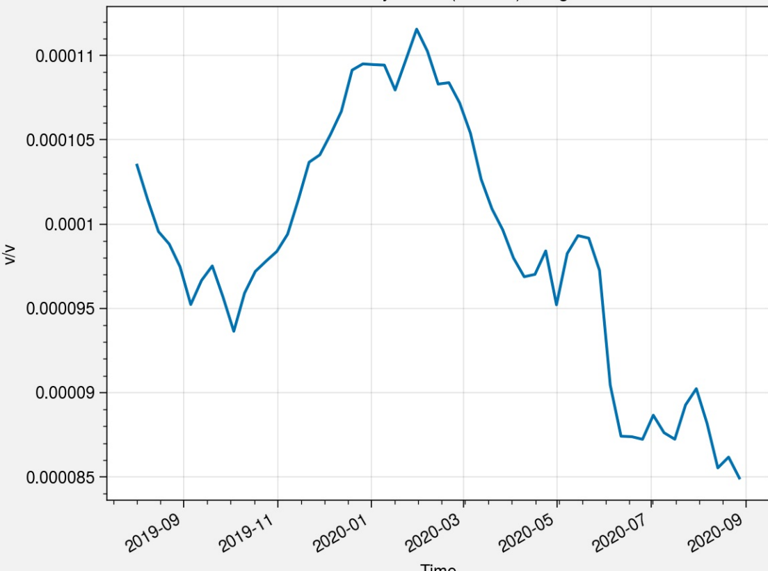
COUniformEmis25dayTracer (surface), region = Global
