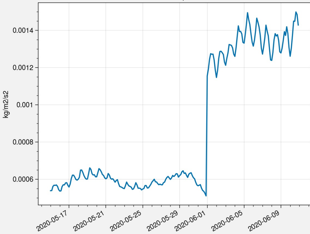
Upward moist convective mass flux: Global full atmosphere mean
