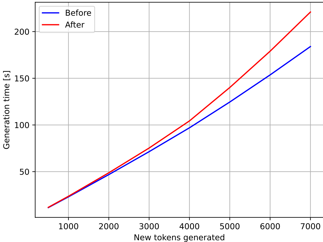
Mistral-7B-v0.1 Input size 300, Batch size 1
