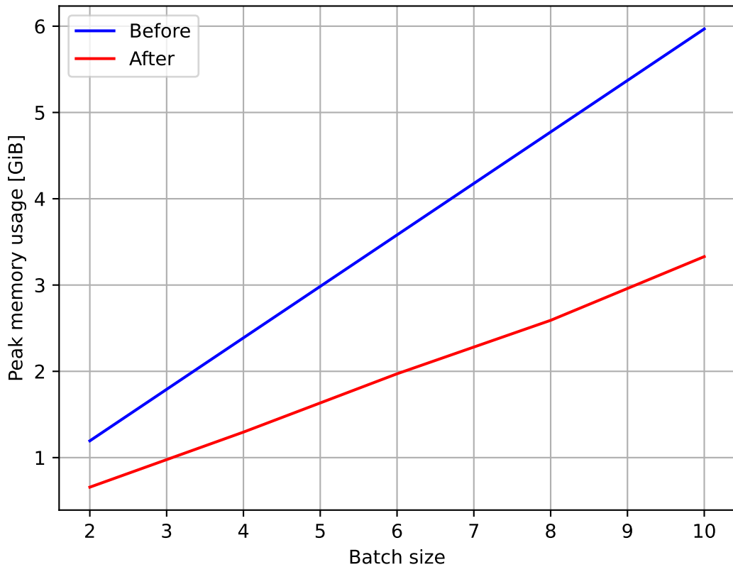
Mistral-7B-v0.1 Input size 300, New tokens 2000
