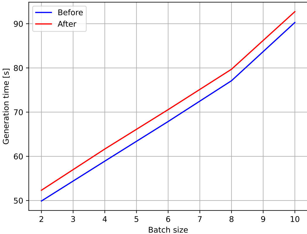
Mistral-7B-v0.1 Input size 300, New tokens 2000
