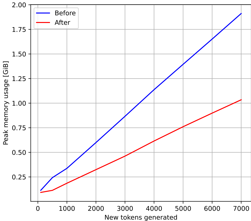
greedy Input size 300, Batch size 1
