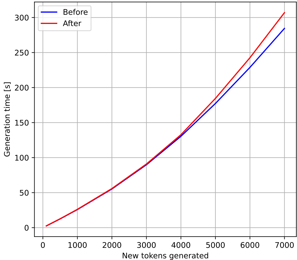
constrained beam search Input size 300, Batch size 1 'num_beams': 2
