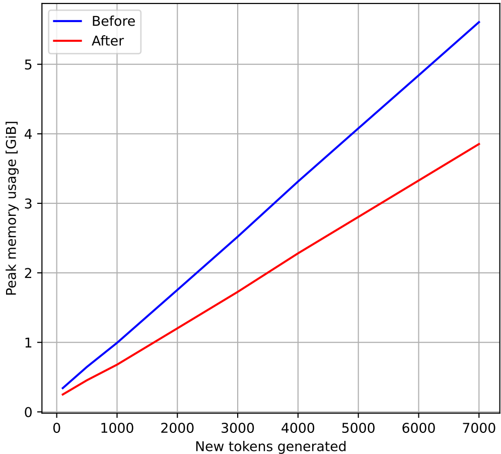
constrained beam search Input size 300, Batch size 1 'num_beams': 2
