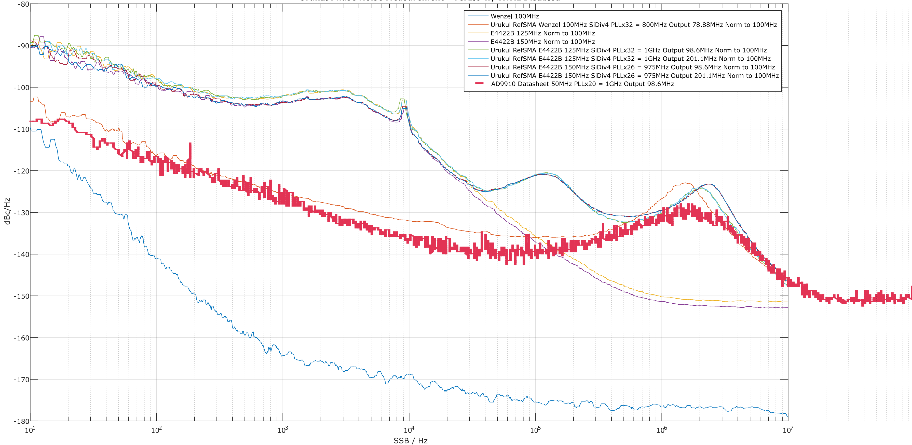
Urukul Phase Noise Measurement - Ver1.0 w/ XTAL Disabled
