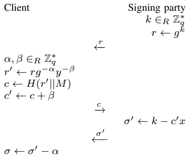
Fig. 1: Blind Schnorr signature protocol to obtain a blind signature (\sigma, c) on message M
