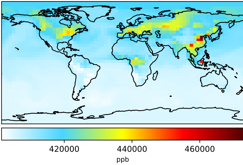
co2_sim (Ref) 4.0x5.0
