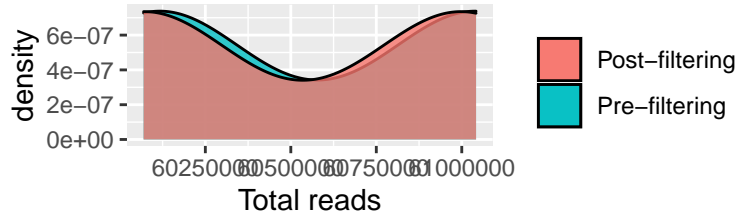
Number of bases across samples
