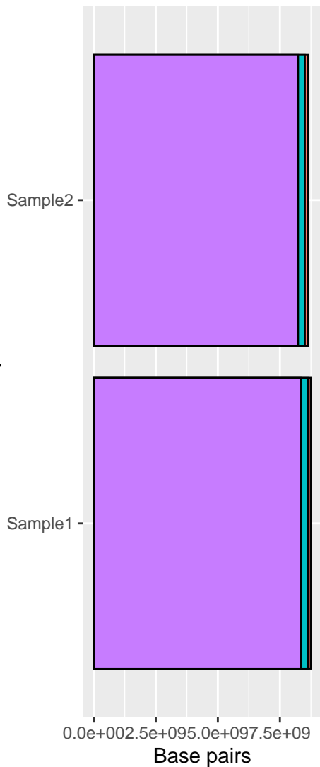
Raw read QC summary stacked bar plot
