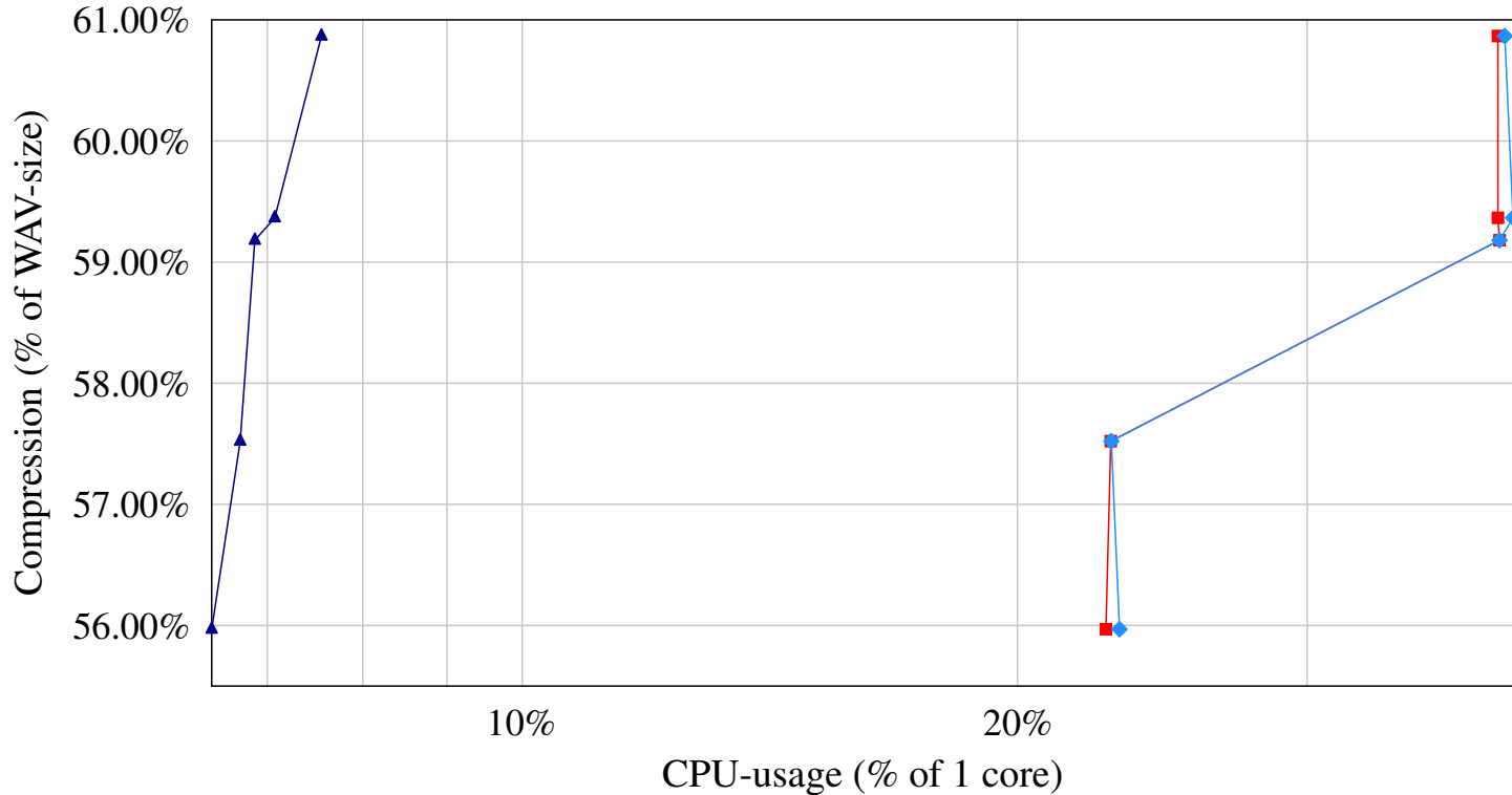
Decoding CPU-usage vs compression for set of 16bit tracks vbuf
