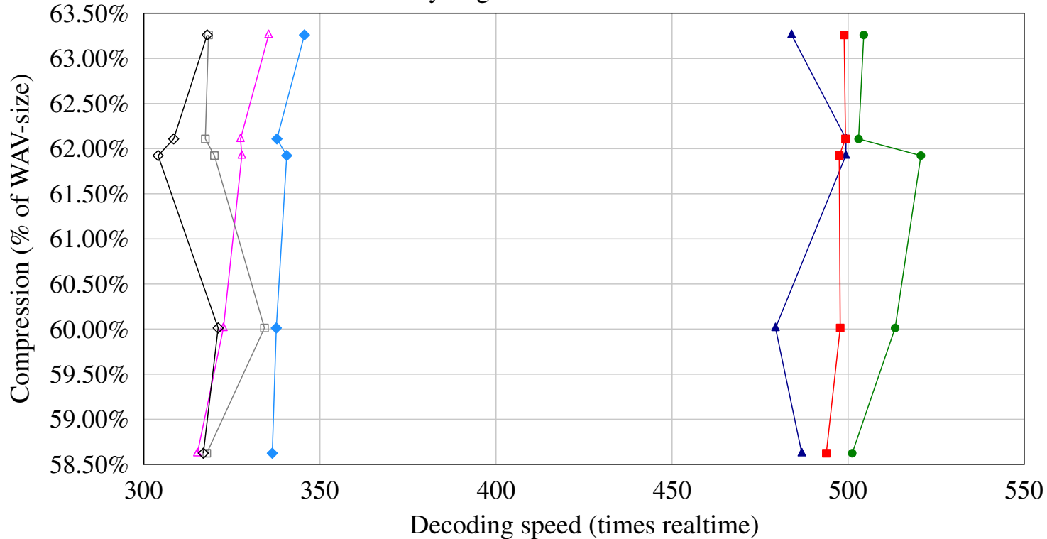
Decoding realtime speed vs compression for very large set of tracks vbuf read HDD
